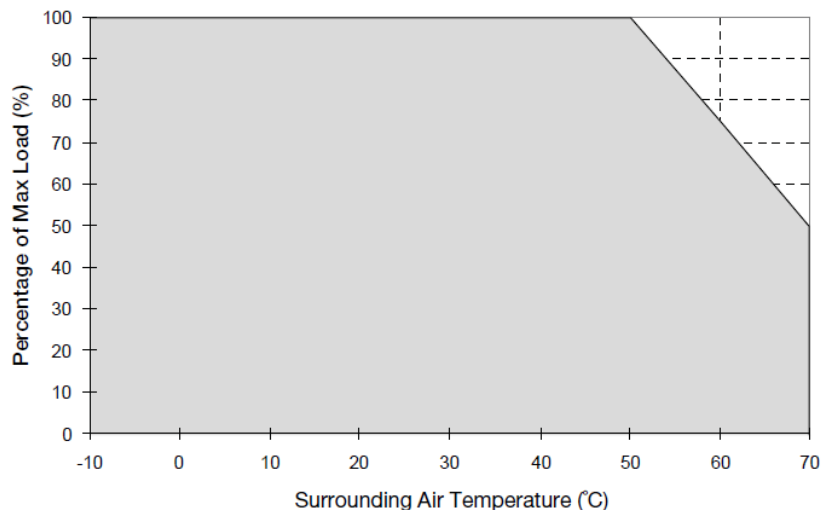
Fig. 1 De-rating for Horizontal Mounting Orientation > 50°C de-rate power by 2.5% / °C
