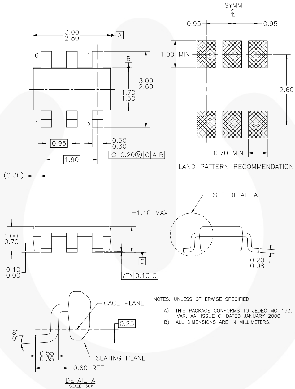
Figure 22. 6-LEAD, SUPERSOT-6, JEDEC MO-193, 1.6 MM WIDE
