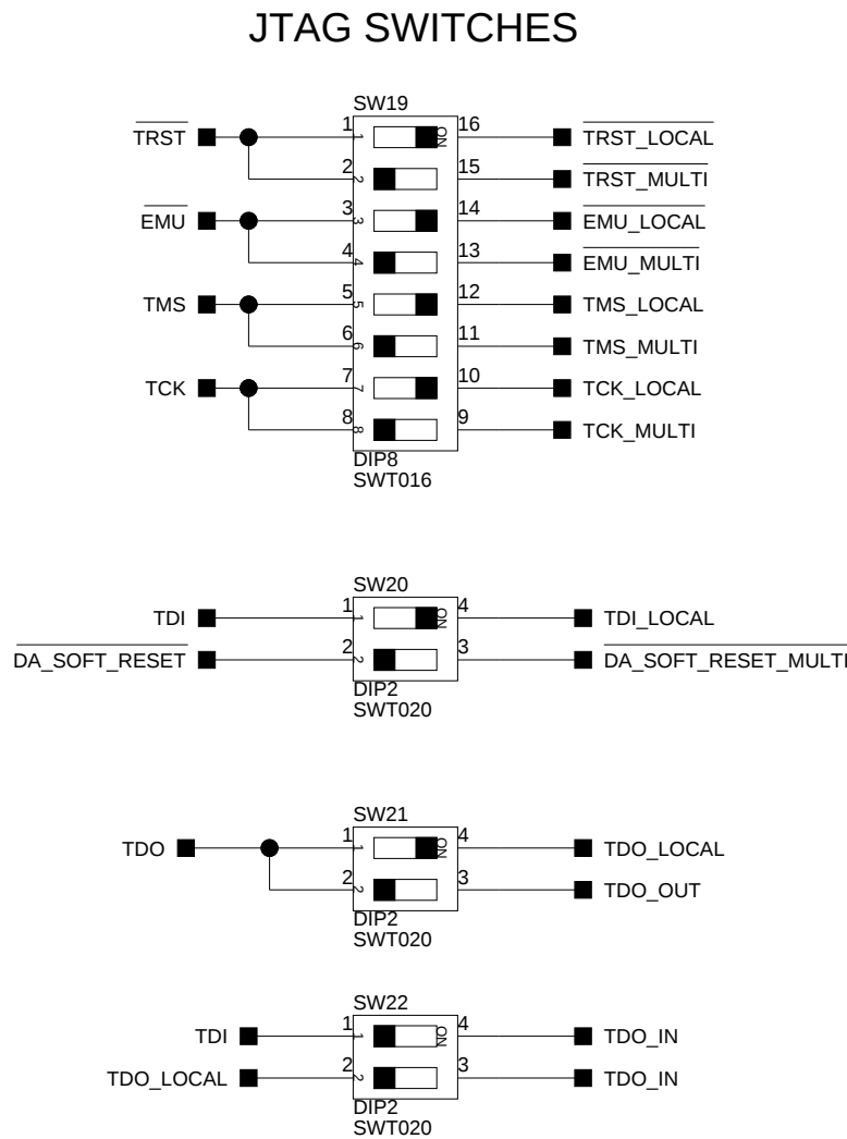
MULTI PROCESSOR JTAG SETTINGS VIA HP-USB EMULATOR USING TWO OR MORE EZ-BOARDS (LINK PORT CABLES REQUIRED FOR MORE THAN TWO BOARDS)
