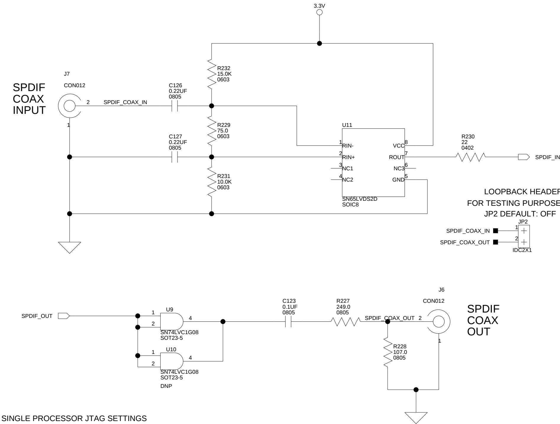
SINGLE PROCESSOR JTAG SETTINGS VIA HP-USB EMULATOR OR DEBUG AGENT (DEFAULT)
