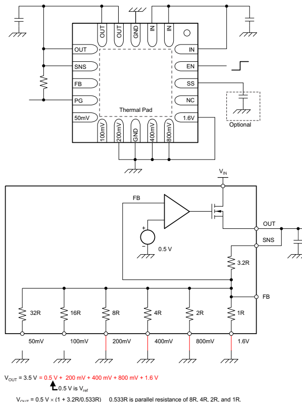
Figure 39. 3.5-V Configuration
