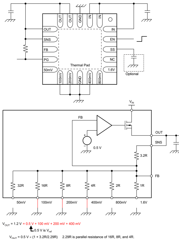
Figure 35. 1.2-V Configuration
