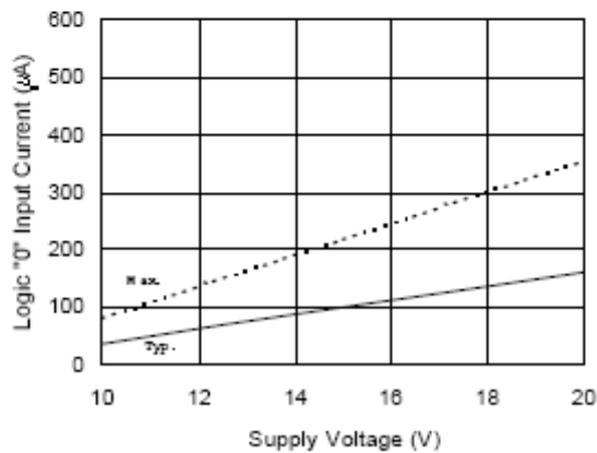
Figure 30B. Logic "0" Input Current vs. Supply Voltage (IR2136/21363/21365 and IR21362 Low Side Only)
