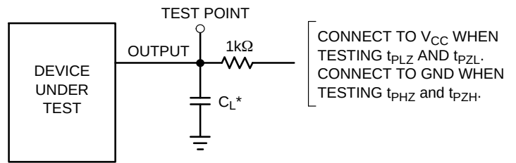
Figure 5. Test Circuit
