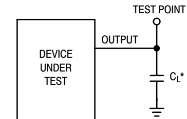
Figure 2. Test Circuit
