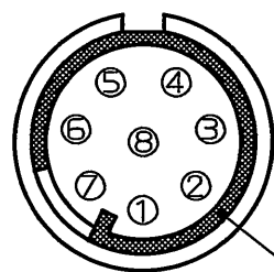
DETAIL B (SCALE 5:1) CONTACT ARRANGEMENT
