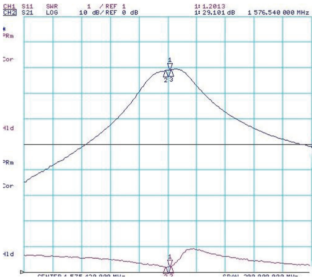
S21: LNA Gain
