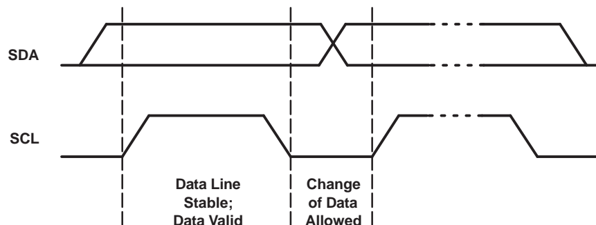
Figure 20. Bit Transfer
