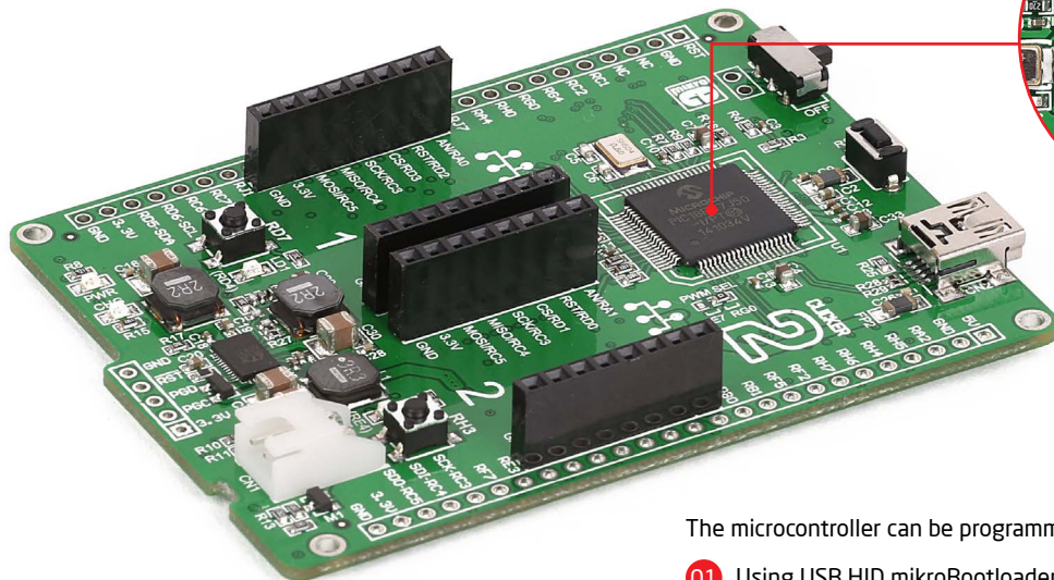
Figure 3-1: PIC18F87J50 microcontroller
