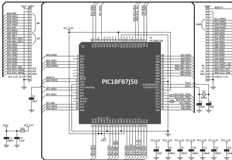
Figure 8-1: Connecting pads schematic
