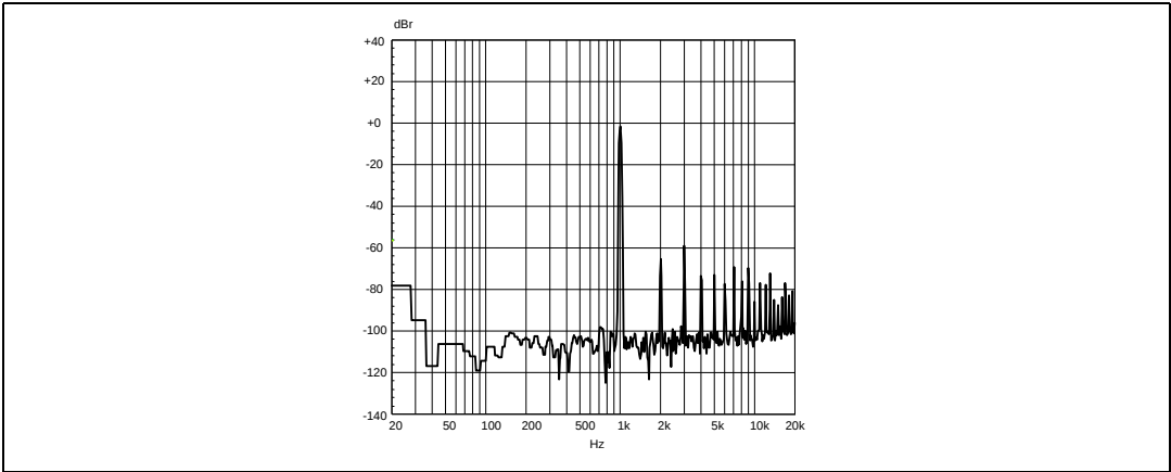
Figure 26. FFT 0 dBFS 1 kHz, 6 \Omega
