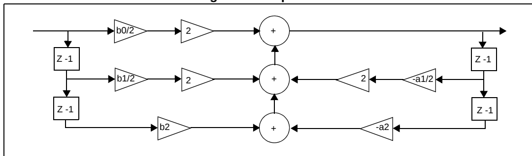
Figure 49. Biquad filter
