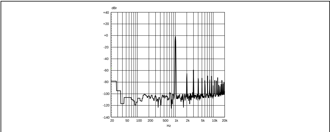
Figure 27. FFT 0 dBFS 1 kHz, 4 \Omega
