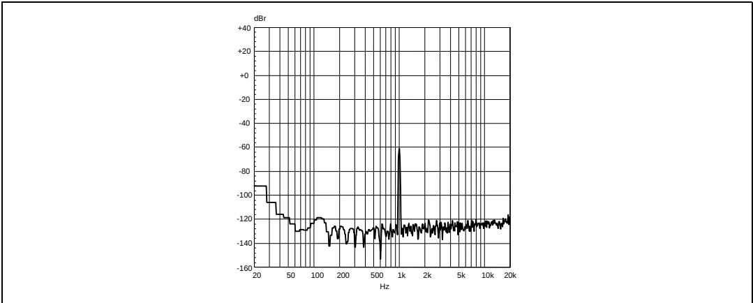
Figure 28. FFT -60 dBFS 1 kHz, 8 Ω
