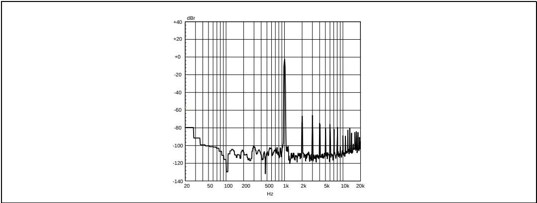
Figure 25. FFT 0 dBFS 1 kHz, 8 \Omega
