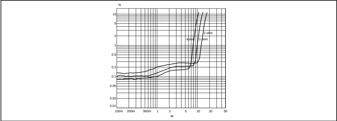
Figure 34. THD+N vs. output power, single ended, 1 kHz, half-bridge binary
