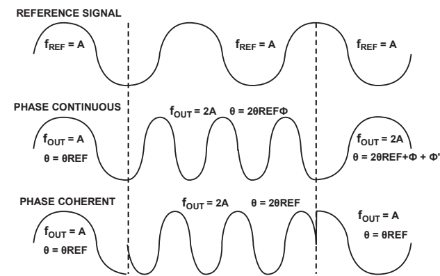
Figure 31. Difference Between a Phase Continuous Frequency Change and a Phase Coherent Frequency Change
