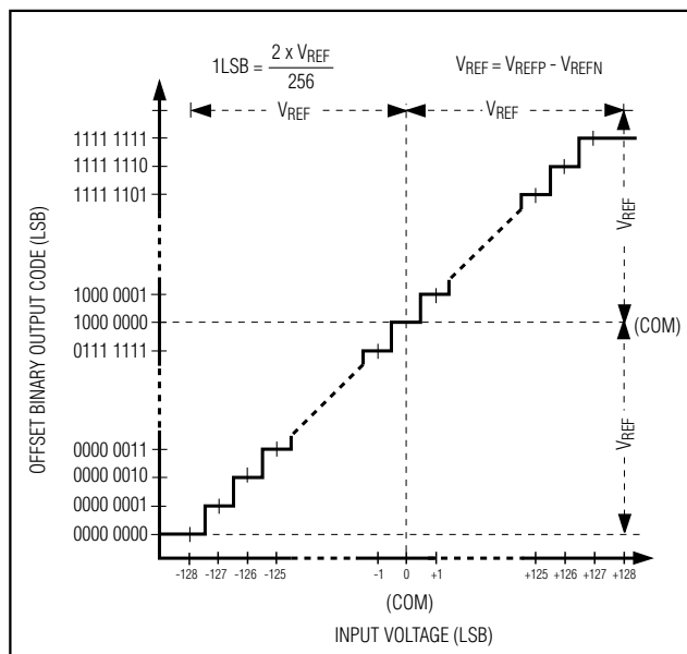
Figure 6. Transfer Function
