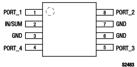
Figure 2. PD4W09-59LF Pinout – 8-Pin MSOP-8 (Top View)
