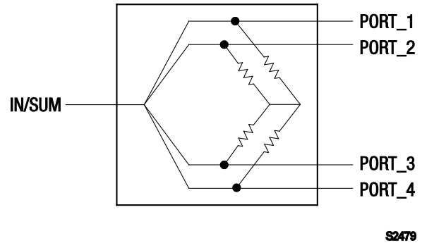
Figure 1. PD4W09-59LF Block Diagram
