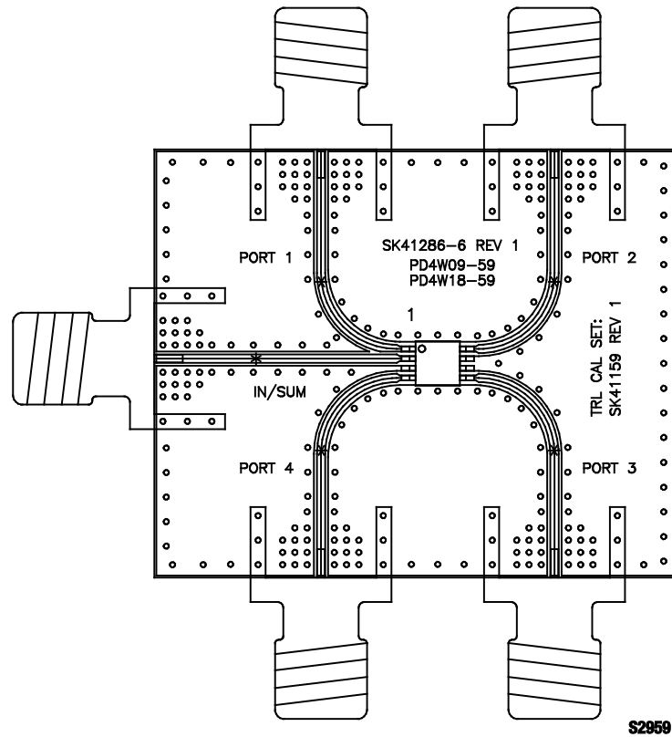
Figure 9. PD4W09-59LF Evaluation Board Assembly Drawing
