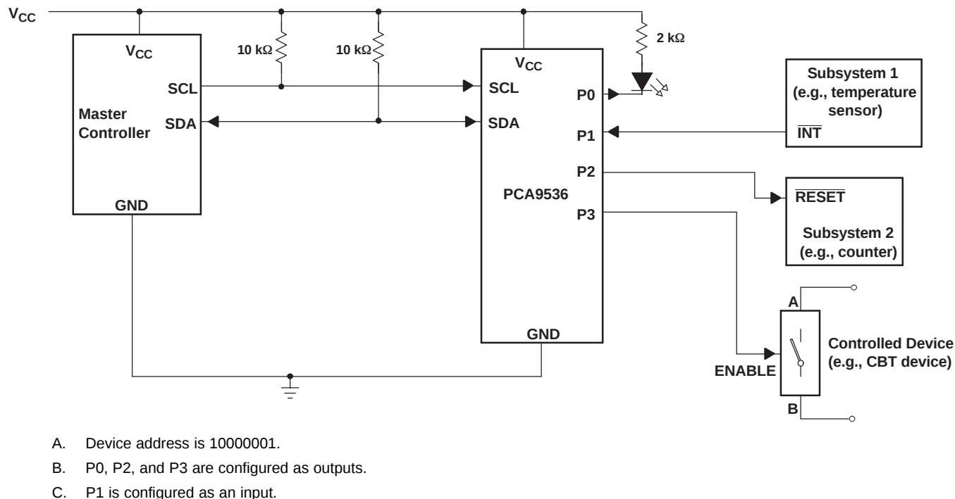
Figure 27. Typical Application
