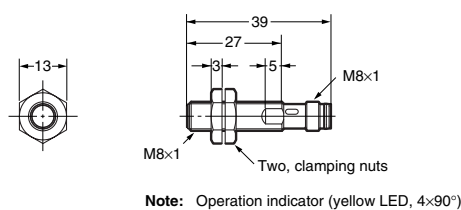
E2A-S08LS02-M5-□□
