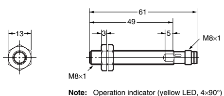
E2A-S08LS02-M5-□□
