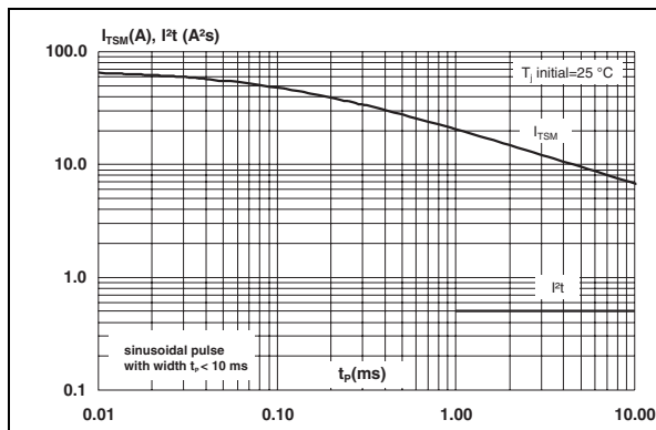
Figure 12. Non repetitive surge peak on-state current and corresponding value of I²t
