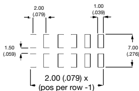
Recommended PCB layouts
