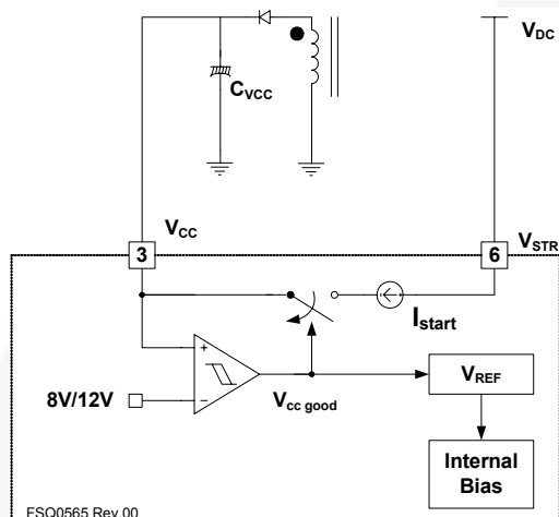
Figure 23. Startup Circuit
