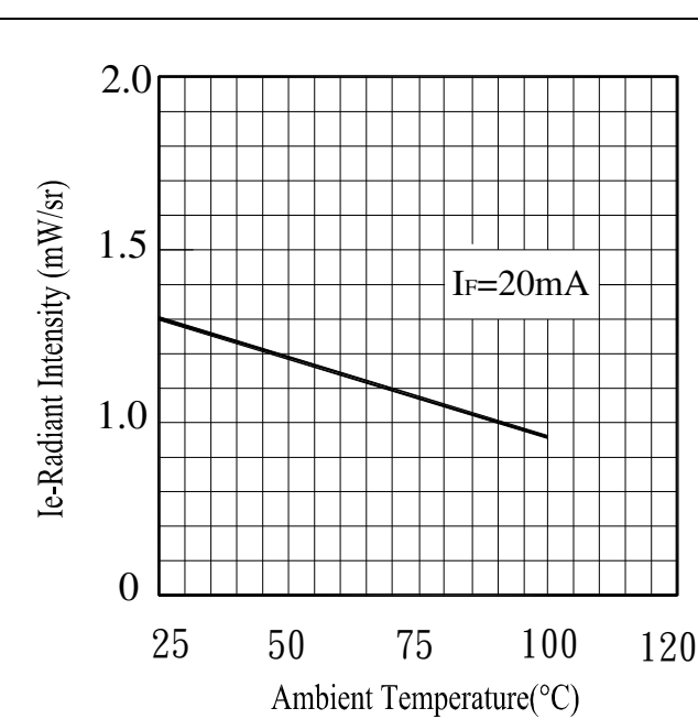
Relative Intensity vs Ambient Temperature(°C)
