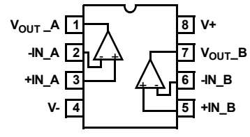
ISL28208 (8 LD MSOP, SOIC) TOP VIEW
