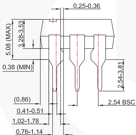
Figure 11. 6-pin DIP Through Hole
