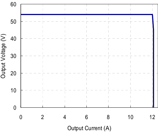
Figure 13: Output voltage vs. load current showing typical current limit curves and converter shutdown points.
