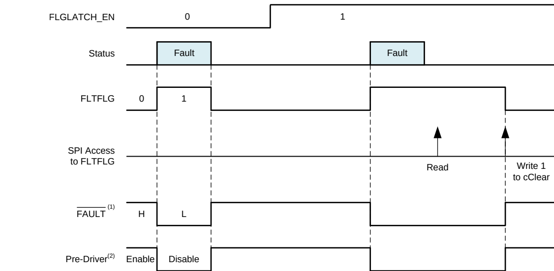
Figure 9. FLGFLG and FLGLATCH_EN
