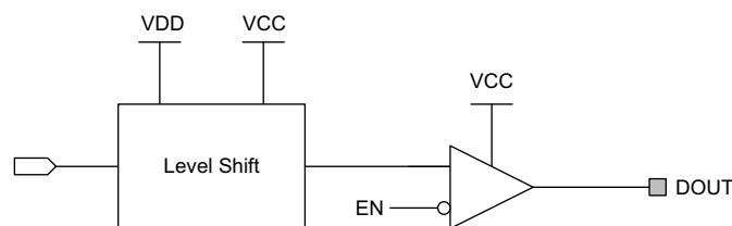
Figure 25. Output Buffer2 Block Diagram
