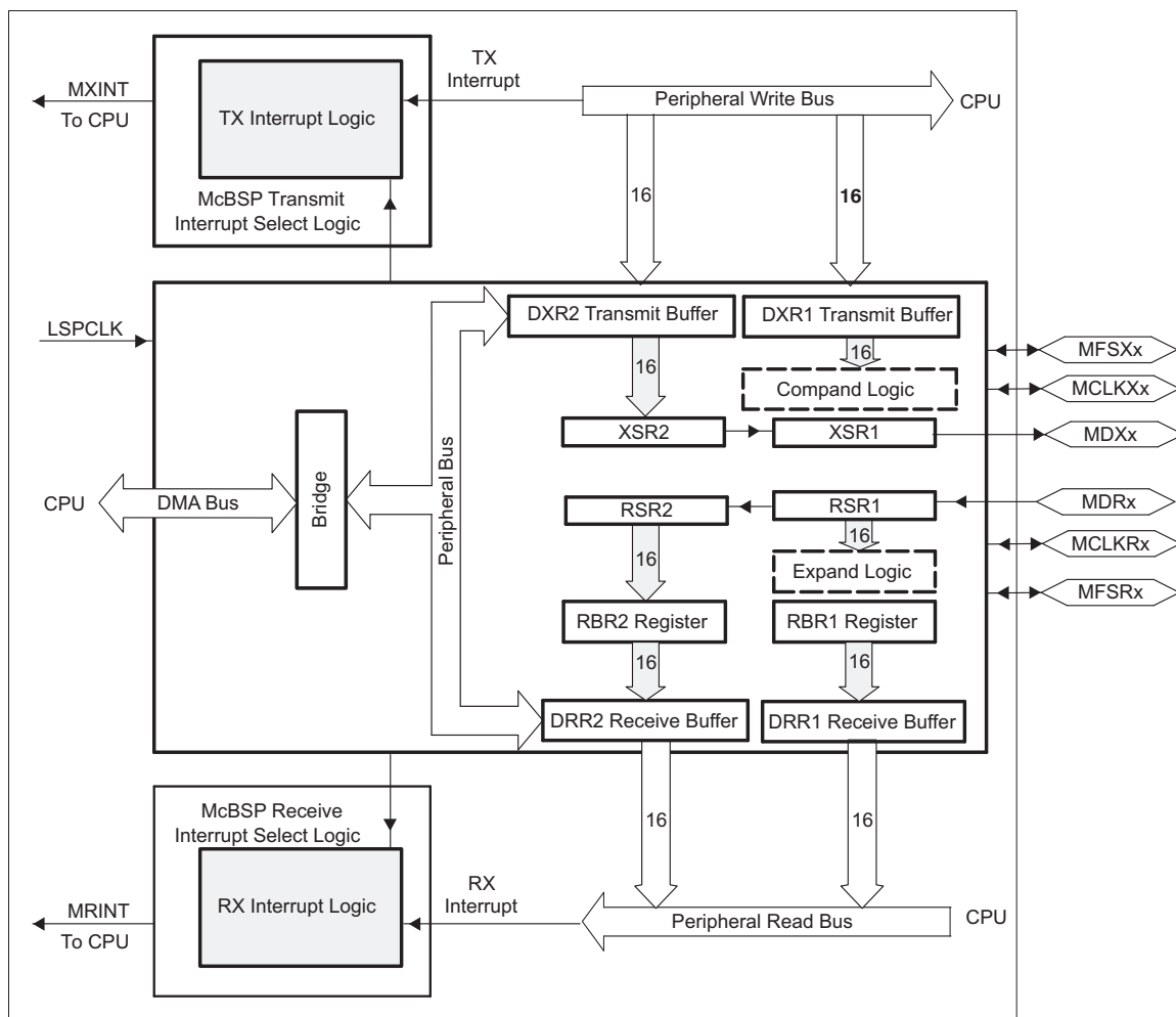
Figure 6-37. McBSP Module
