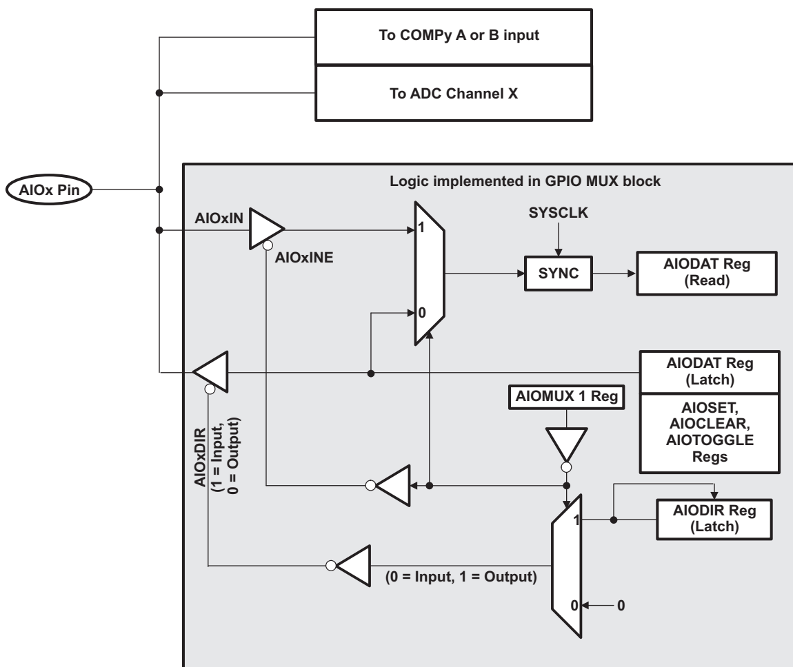
Figure 6-28. AIOx Pin Multiplexing
