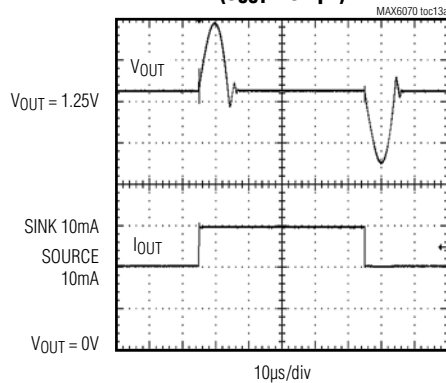
MAX6071_12 \pm 10\text{mA} LOAD TRANSIENT ( C_{OUT} = 0.1\mu\text{F} )
