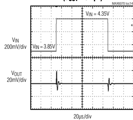
MAX6070_12 LINE TRANSIENT ( C_{OUT} = 0.1\mu\text{F} )
