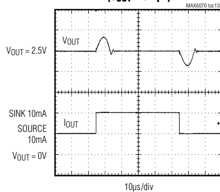
MAX6071_25 \pm 10\text{mA} LOAD TRANSIENT ( C_{OUT} = 0.1\mu\text{F} )
