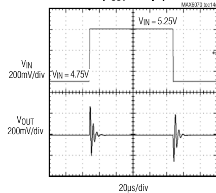
MAX6070_41 LINE TRANSIENT ( C_{OUT} = 0.1\mu\text{F} )
