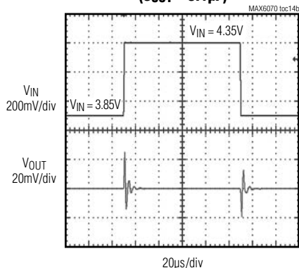
MAX6070_25 LINE TRANSIENT ( C_{OUT} = 0.1\mu\text{F} )
