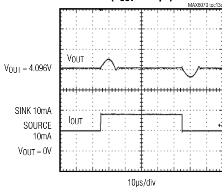
MAX6071_41 \pm 10\text{mA} LOAD TRANSIENT ( C_{OUT} = 0.1\mu\text{F} )
