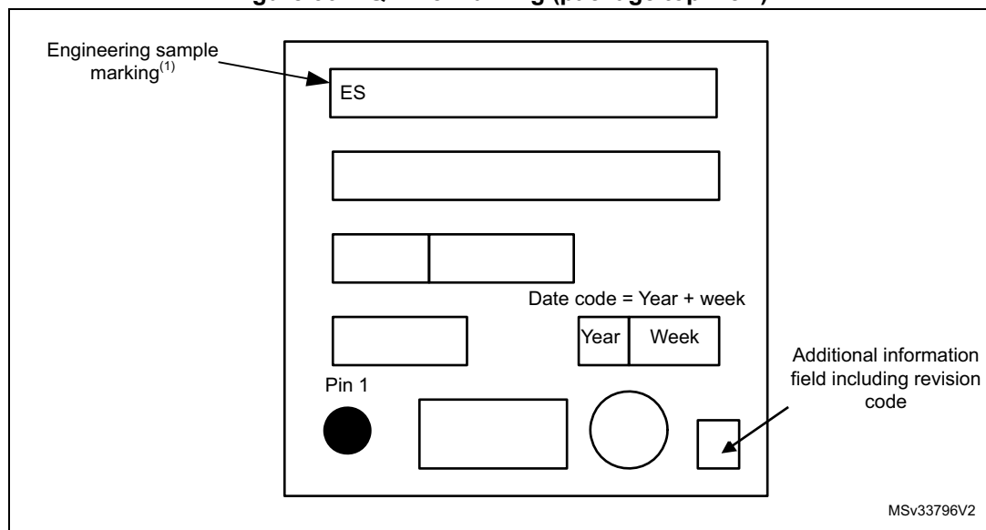
Figure 36. LQFP48 marking (package top view)
