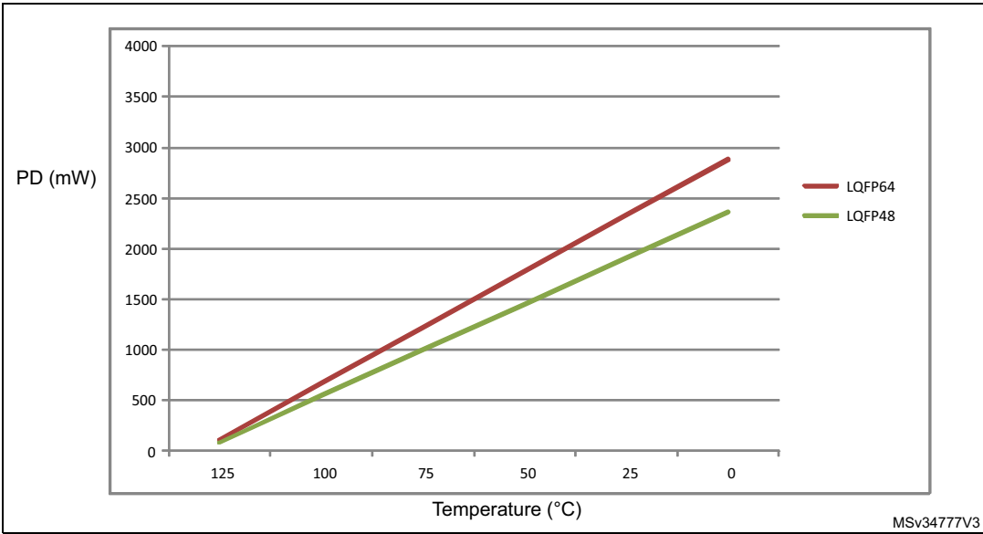
Figure 40. Thermal resistance
