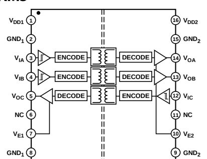
Figure 2. ADuM1301 Functional Block Diagram
