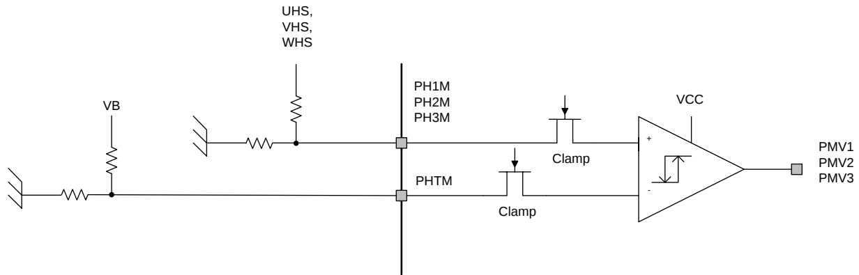
Figure 14. Phase Comparator Block Diagram
