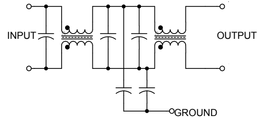
Figure 4. Internal Schematic
