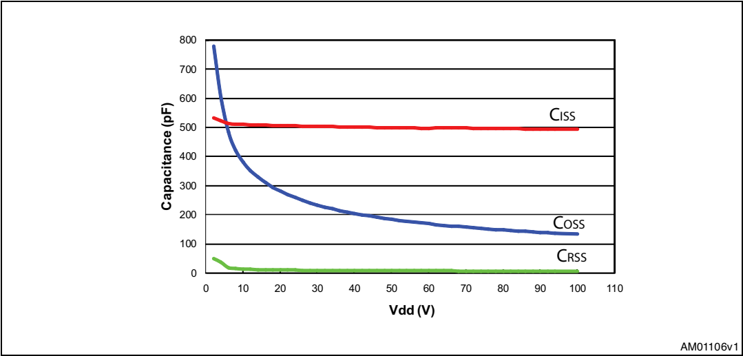
Figure 6. Capacitances vs. drain supply voltage
