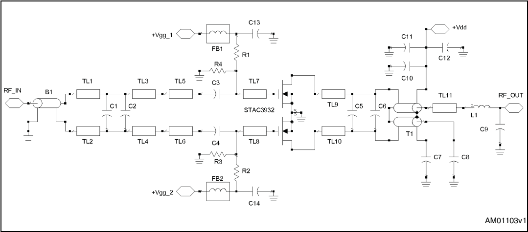
Figure 3. Electrical schematic
