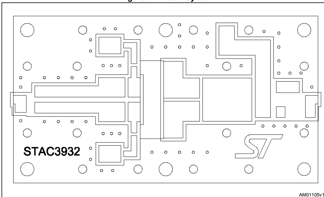
Figure 5. Circuit layout
