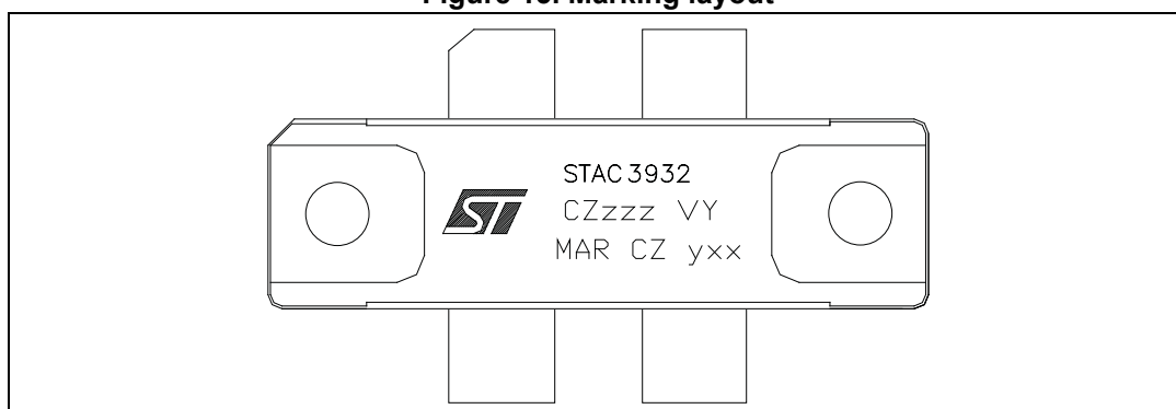
Figure 15. Marking layout
