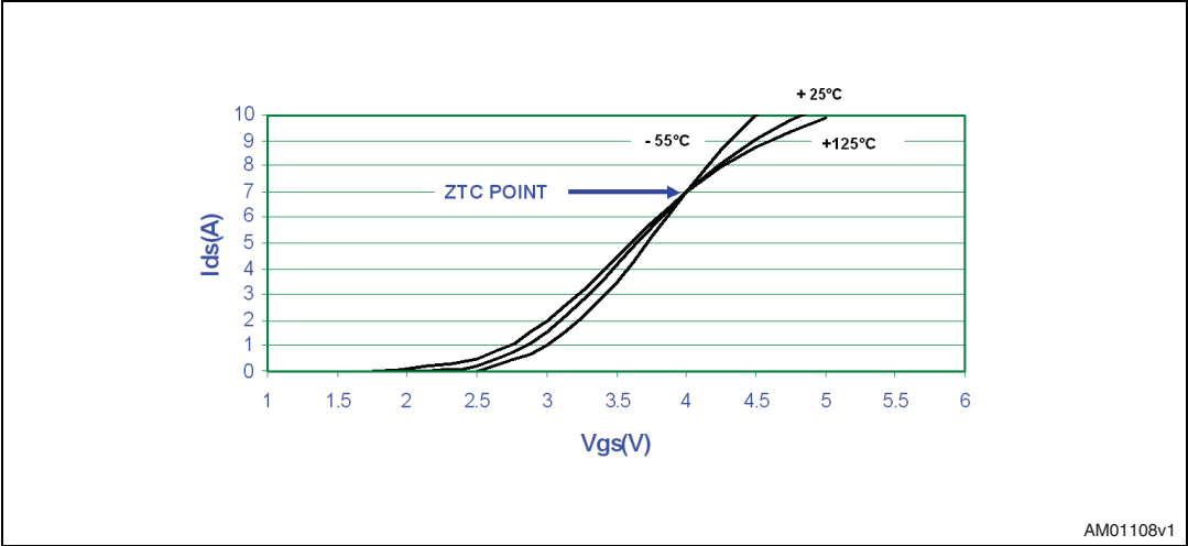
Figure 10. Zero temperature coefficient point
