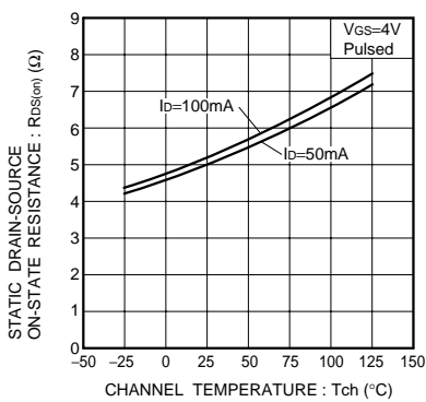
Fig.15 Static drain-source on-state resistance vs. channel temperature
