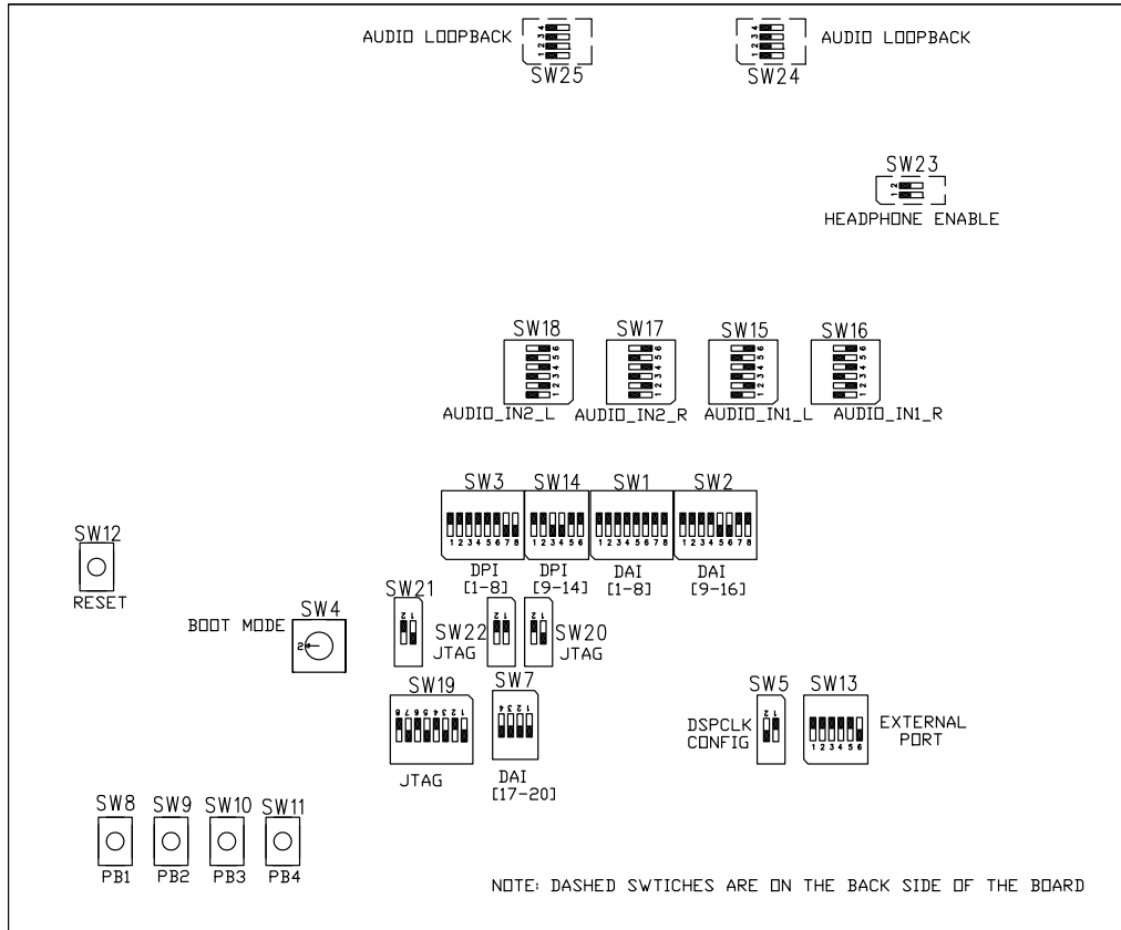
Figure 2-2. Push Button and Switch Locations
