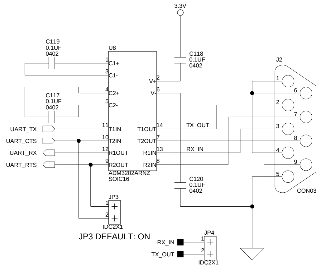
LOOPBACK HEADER FOR TESTING PURPOSES ONLY JP4 DEFAULT: OFF
