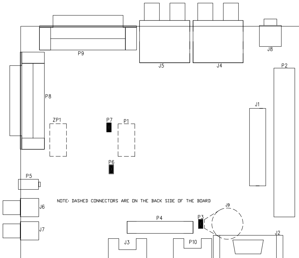
Figure 2-5. Connector Locations
