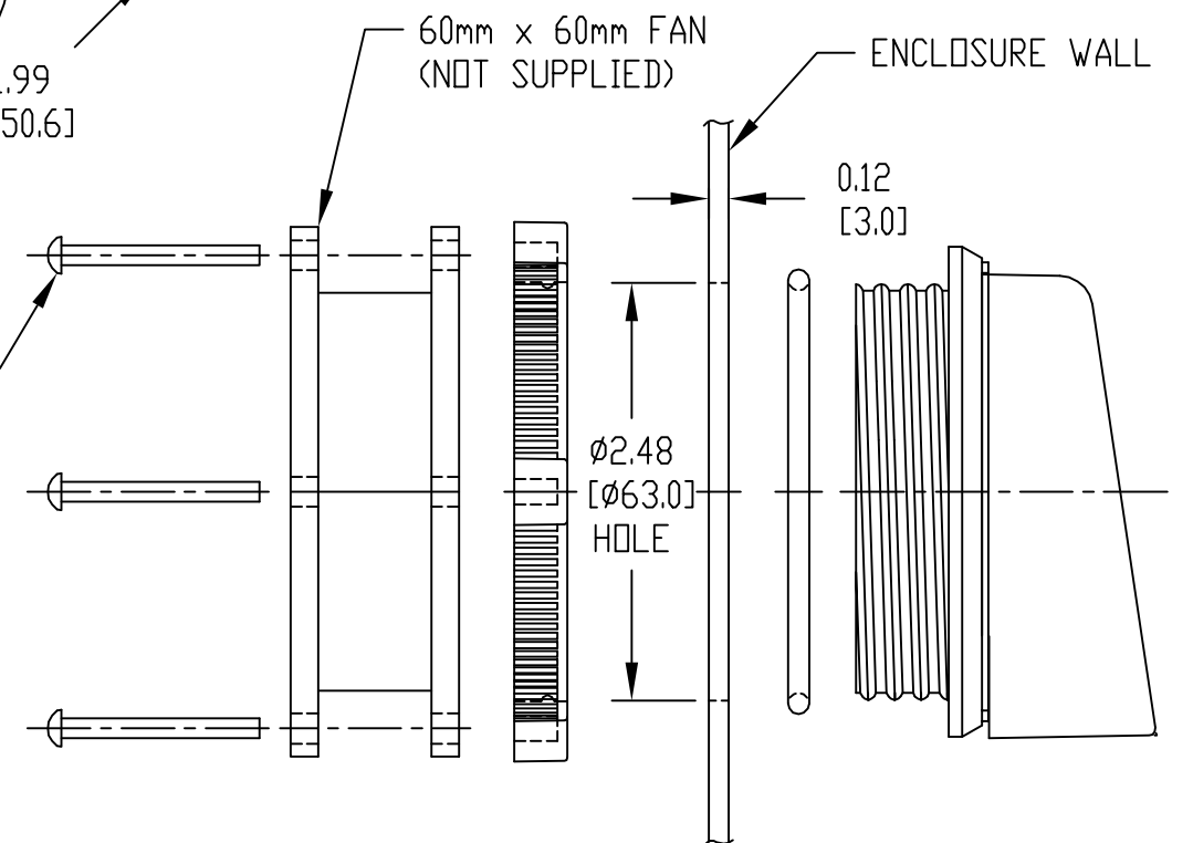
TYPICAL INSTALLATION
