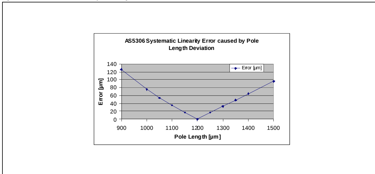
Figure 9. Additional Error Caused by Pole Length Variation: AS5306
