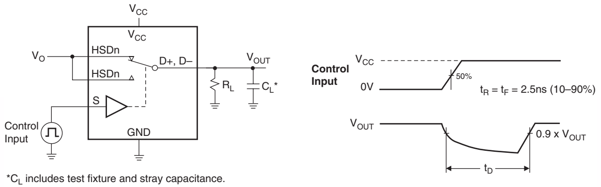
Figure 14. Break-Before-Make (t BBM )
