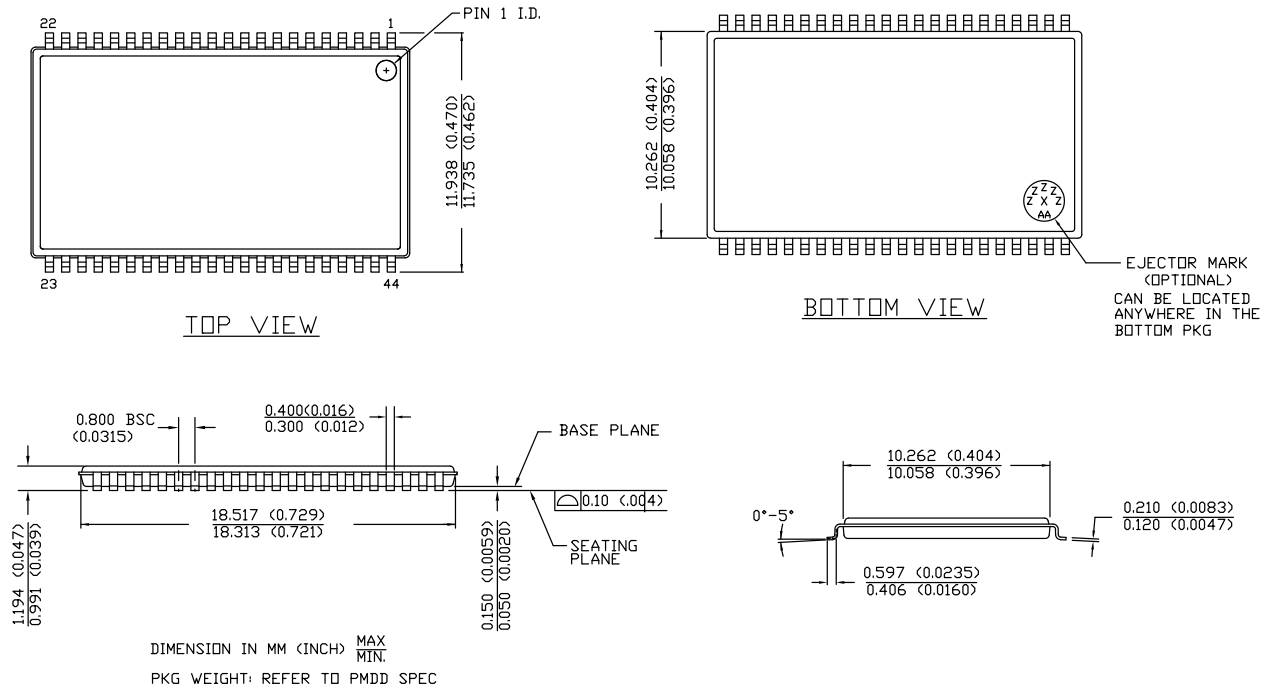
Figure 8. 44-Pin TSOP II
