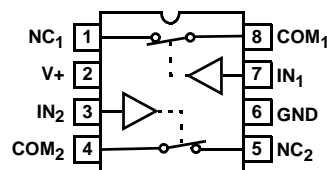
ISL84542 (SOT-23) TOP VIEW
