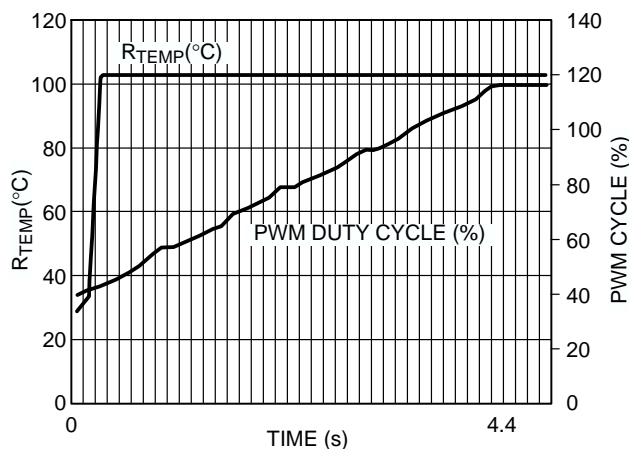
Figure 78. Enhanced Acoustics Mode with Ramp Rate = 8
