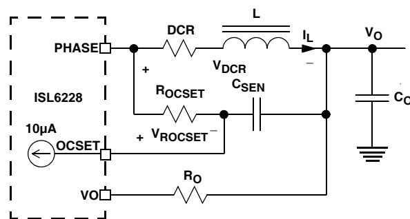
FIGURE 5. OVERCURRENT-SET CIRCUIT
