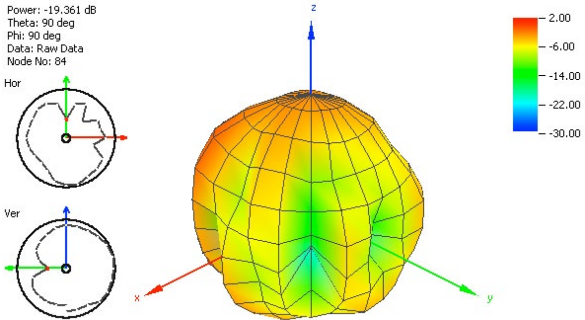
Figure 31. Radiation Pattern at 2450 MHz of FXUB70 Port 2.
