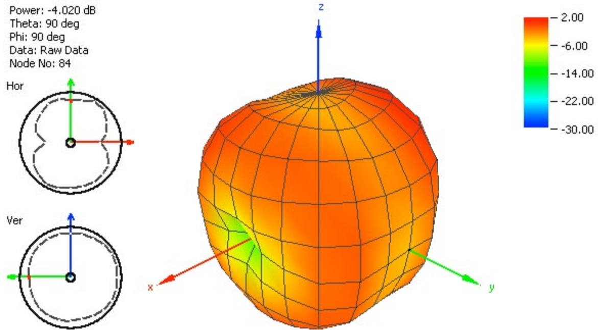
Figure 21. Radiation Pattern at 1575 MHz of FXUB70 Port 2
