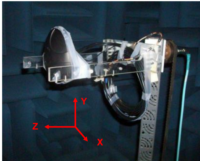
MA. 671 tested in CTIA approved 3D chamber
