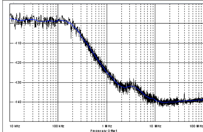
200-kHz Loop Bandwidth Figure 4-15. Phase Noise 869.5 MHz (10-kHz to 100-MHz Offset)
