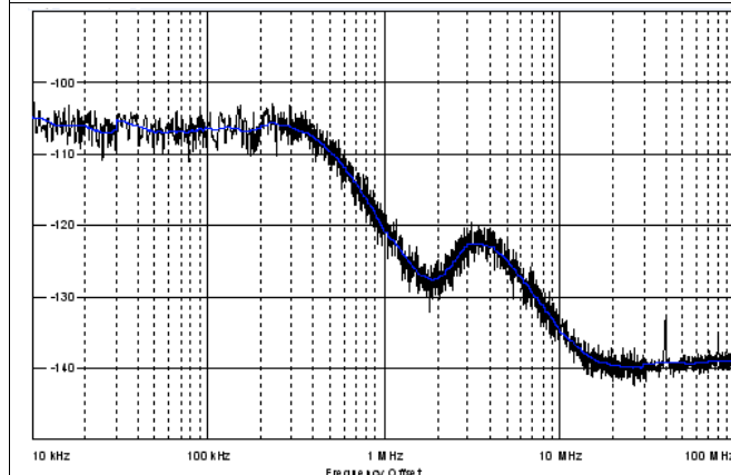
400-kHz Loop Bandwidth Figure 4-17. Phase Noise 869.5 MHz (10-kHz to 100-MHz Offset)
