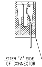
SINGLE ROW
