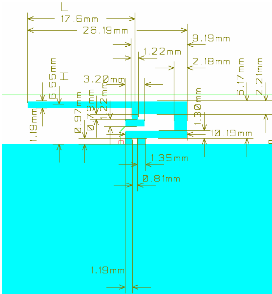
Figure 2: Antenna dimensions
