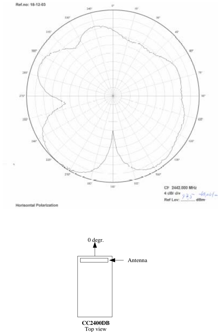
Figure 3: Radiated pattern horizontal mounting
