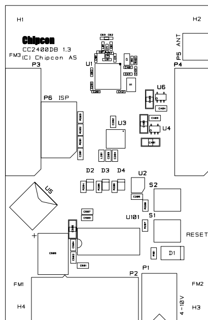
Top Assembly
