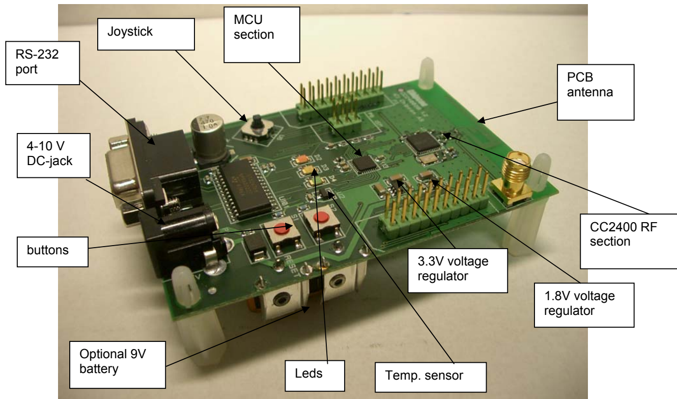
Figure 1: CC2400DB overview
