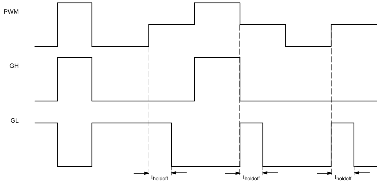
Figure 5. Tri-State Operation
