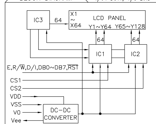
BLOCK DIAGRAM 1/64 DUTY, 1/6 BIAS
