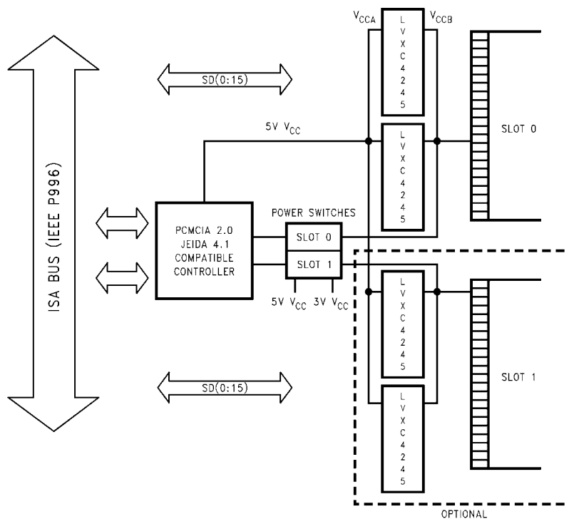
Block Diagram
