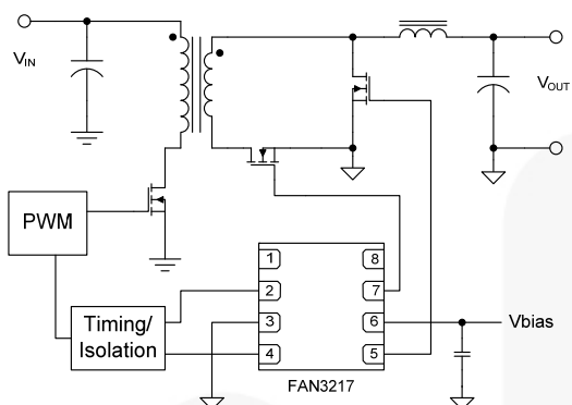
Figure 36. Forward Converter with Synchronous Rectification
